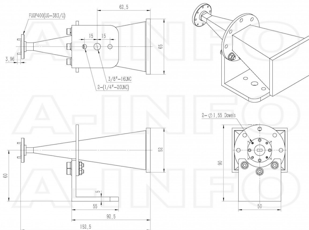
FUGP400 Output with L Type Mounting Bracket & Radome (Option, P/N: LB-22-25-L2 & LB-22- 25-A2SPO, Outdoor Application)
